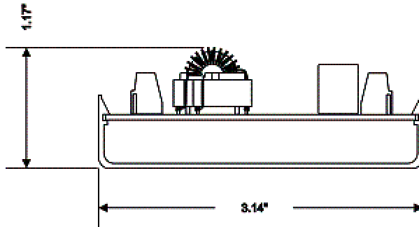
APC-SCR-CM-1 MODULE (MOUNTED IN SNAP TRACK)
