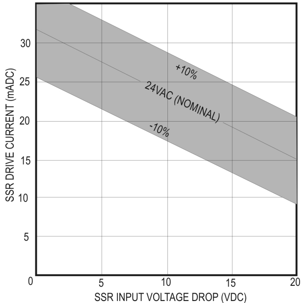
APC-SCR-CM-1's Output Drive Current vs. SSR Input Voltage Drop
